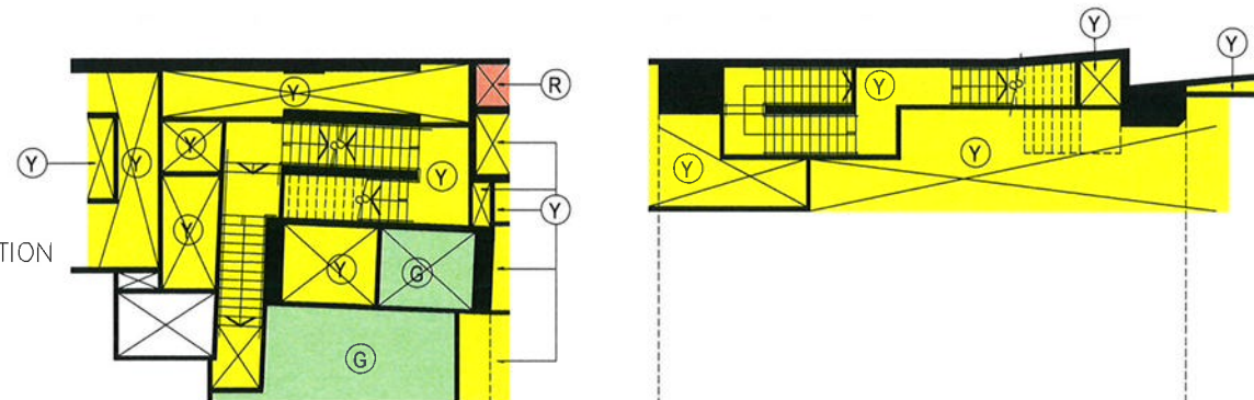
PART PLAN OF STAIRCASE '1' AT LEVEL +21.875
