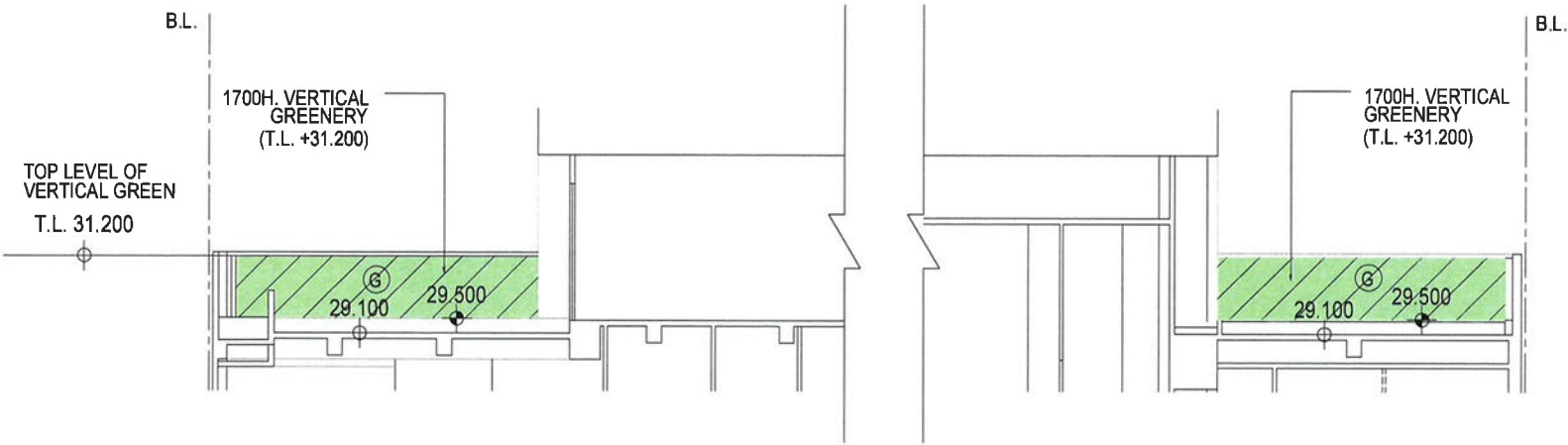
ELEVATION 'B' OF VERTICAL GREENERY AT 2/F RESIDENTIAL COMMON AREAS AND FACILITIES 1 : 100
