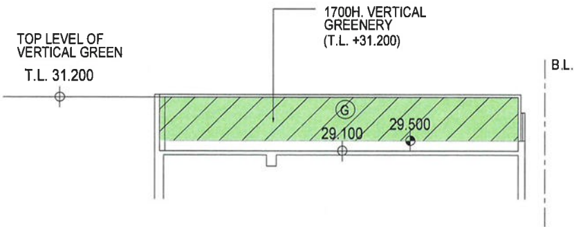
ELEVATION 'C' OF VERTICAL GREENERY AT 2/F RESIDENTIAL COMMON AREAS AND FACILITIES 1 : 100
